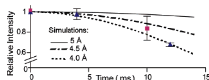
Figure 1. 13 C detect REDOR dephasing ( S/S 0 vs dephasing time) for 13 C–G 8 / 15 N–V 12 p1-COOH (squares) and 13 C–I 16 / 15 N–V 20 p1-COOH (triangles) in hydrated 3:1 DTPC/DTPG at 1:20 peptide-to-lipid ratio, and T = –50 °C.
