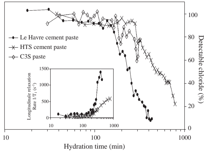
Fig. 2. ^{35}\text{Cl} kinetics of hydration for a cement paste ( \times for HTS and \bullet for Le Havre) and a \text{C}_3\text{S} paste ( \diamond ) produced with an addition 3% of NaCl in mass of cement ( w/c = 0.35 ). Compared to the ^{23}\text{Na} kinetics, the decrease in detectable ^{35}\text{Cl} occurs faster and the increase of the relaxation rate is less pronounced. From the ^{35}\text{Cl} point of view, the amount of \text{C}_3\text{A} is determinant respect to the hardening process.
